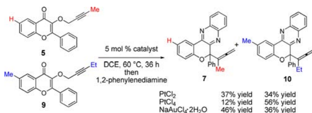
Scheme 1. Crossover Experiments
