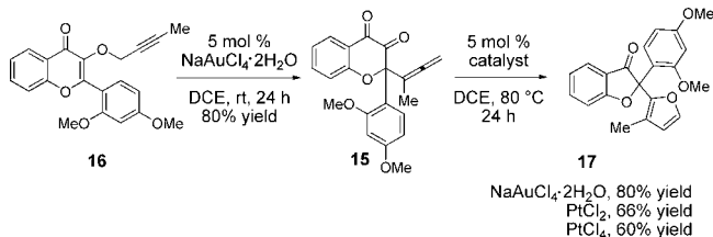
Scheme 4. Preparation and Rearrangement of an Allenyl Chromanedione
