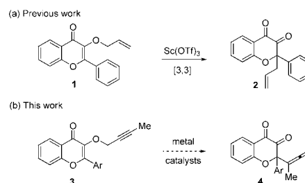
Figure 1. Metal-catalyzed rearrangement of 3-flavone ethers.
