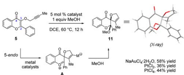
Scheme 2. Intermolecular Trapping of an Oxocarbenium Intermediate
