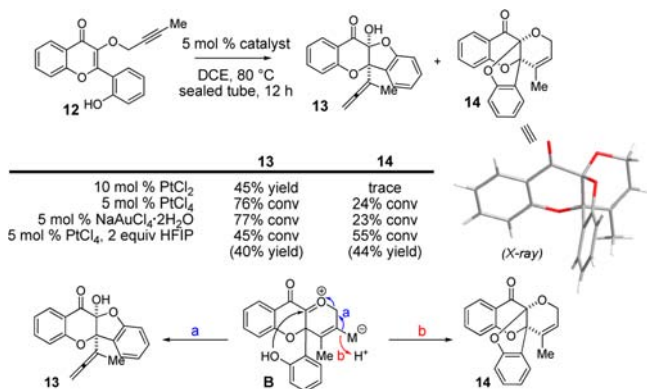
Scheme 3. Intramolecular Trapping of an Oxocarbenium Intermediate
